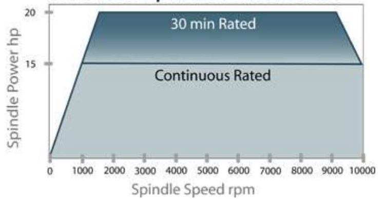
VMC1020 Spindle Power Chart
